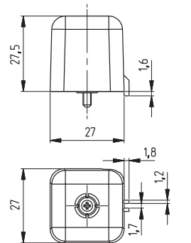
Contact safety guard with PT screw Cable exit AMP1 or AMP2
