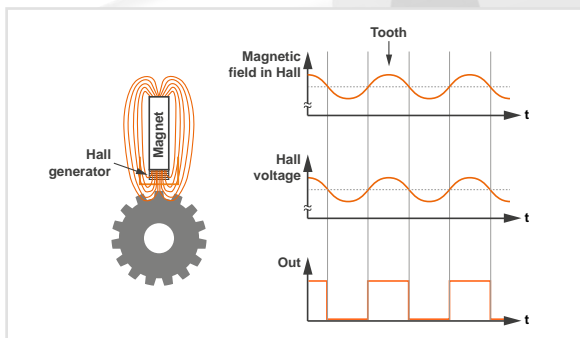
Principle of operation: Hall
