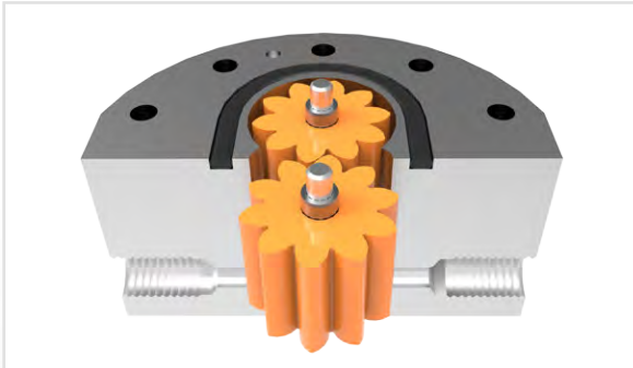
Sectional model
