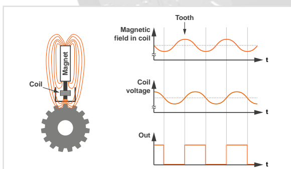
Principle of operation: Inductive
